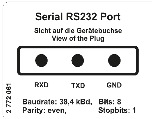
RS232 interface on Tico 774
