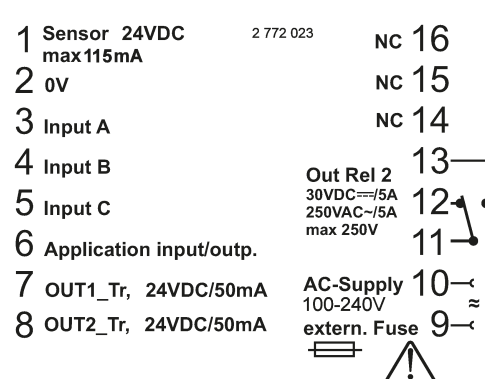
VAC Switch-mode power supply 1 relay/2 transistors
