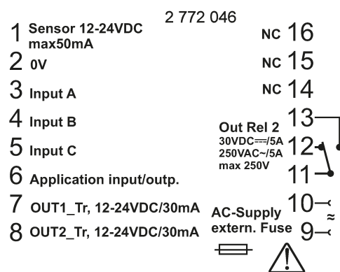
VAC Transformer 1 relay/2 transistors
