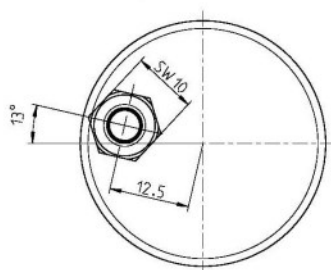
Connection cable axial "A"
